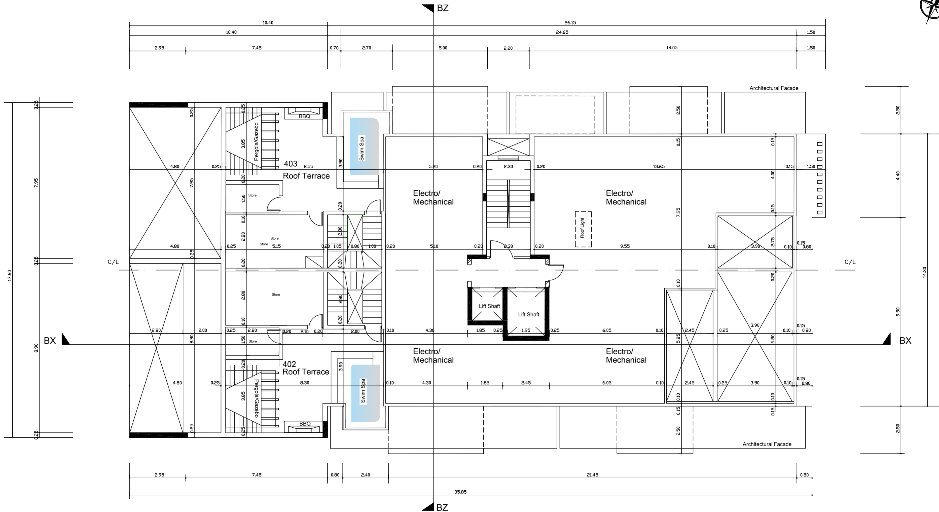
Roof Layout Block B
